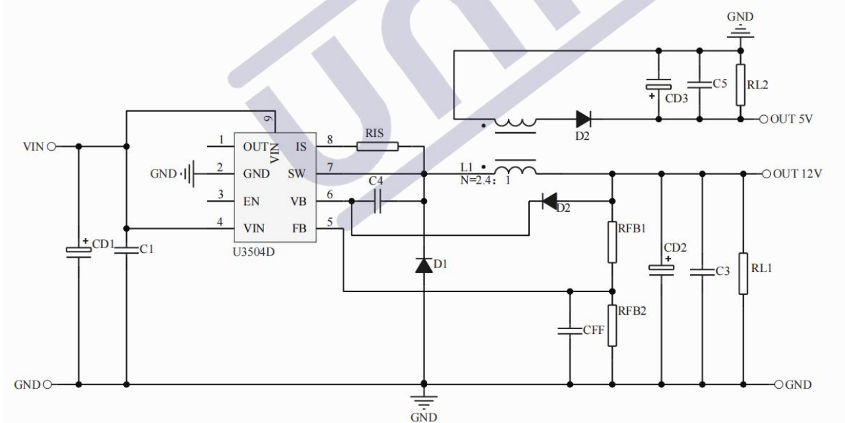
APP4:VOUT12V/VOUT5V
